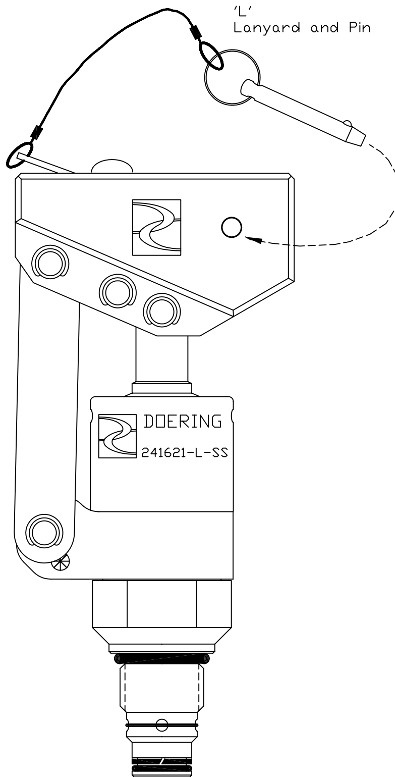
Example Doering Pump with Lanyard & Pin to Join Handle
