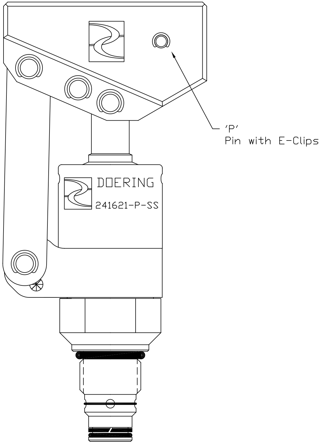
Example Doering Pump with Pin to Join Handle
