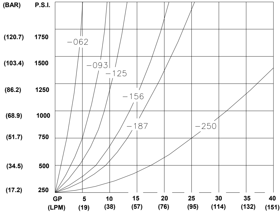
FLOW THRU RESTRICTED ORIFICE
