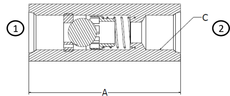
FRF Inline Restrictor Valve
