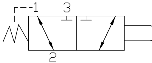
Three Way Spool Valve Functional Symbol Doering Cartridge Valve 1203364
